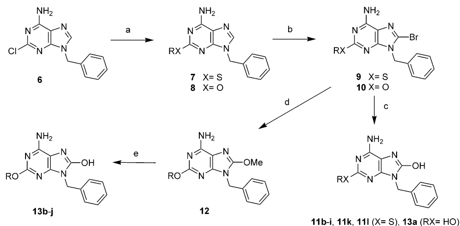
Scheme 1. Reagents and conditions: (a) NaSR, DMF, 110 °C or NaOR, ROH, reflux; (b) Br 2 , CH 2 Cl 2 , rt; (c) 6N HCl, reflux; (d) NaOMe, MeOH, reflux; (e) 12N HCl, rt
