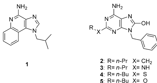
Figure 1. Structures of 1 (Imiquimod) and 2-5 .
