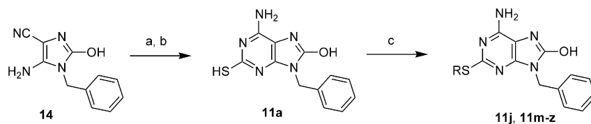
Scheme 1. Reagents and conditions: (a) NaSR, DMF, 110 °C or NaOR, ROH, reflux; (b) Br 2 , CH 2 Cl 2 , rt; (c) 6N HCl, reflux; (d) NaOMe, MeOH, reflux; (e) 12N HCl, rt
